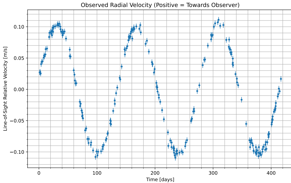
Figure 1: We have isolated the radial velocity of the host star due to the candidate planet. Data begins at UTC 2098-01-13/17:31. Positive values indicate the velocity at which the star is moving towards us; negative indicate the velocity at which it is moving away.
