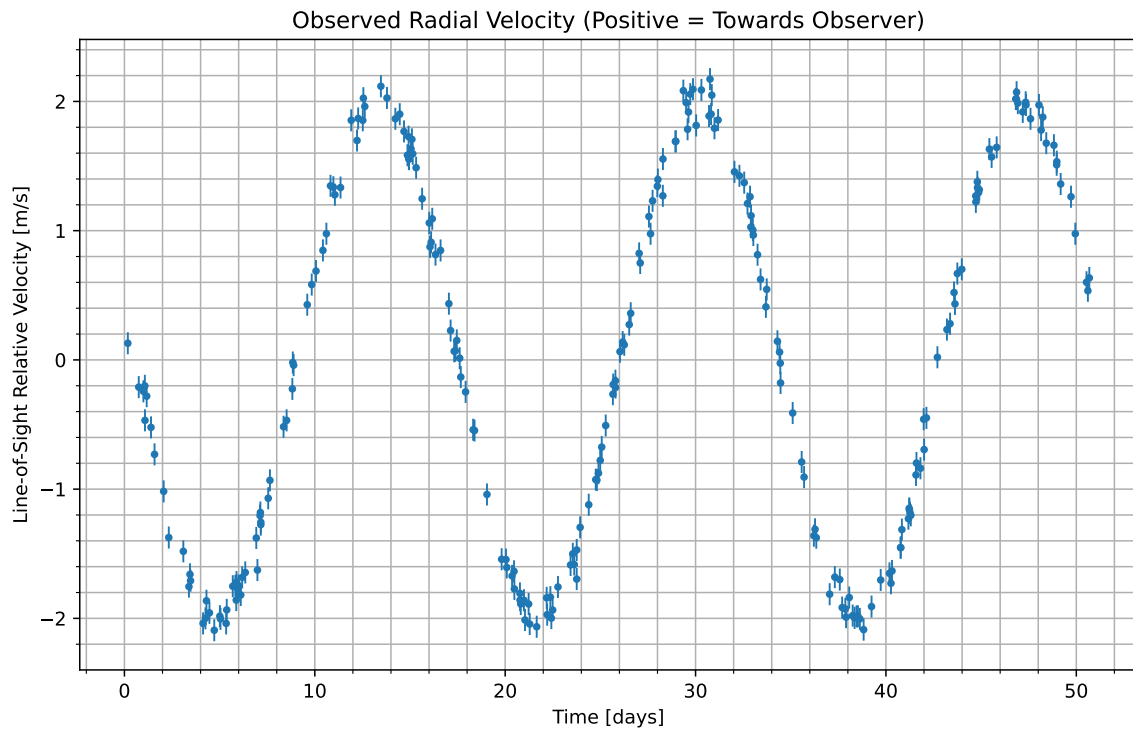
Figure 1: We have isolated the radial velocity of the host star due to the candidate planet. Data begins at UTC 2082-11-26/09:53. Positive values indicate the velocity at which the star is moving towards us; negative indicate the velocity at which it is moving away.
