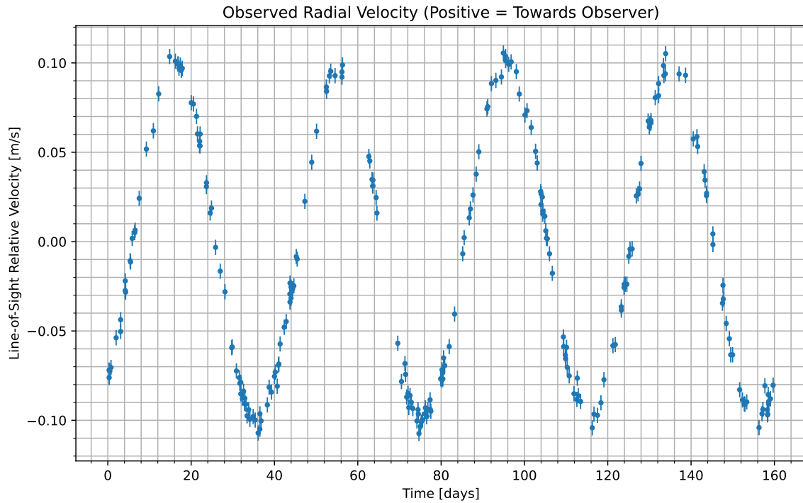
Figure 1: We have isolated the radial velocity of the host star due to the candidate planet. Data begins at UTC 2071-07-05/04:08. Positive values indicate the velocity at which the star is moving towards us; negative indicate the velocity at which it is moving away.
