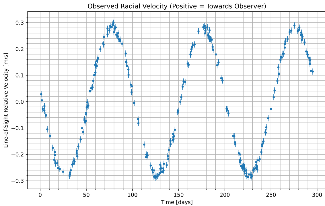
Figure 1: We have isolated the radial velocity of the host star due to the candidate planet. Data begins at UTC 2076-08-24/00:41. Positive values indicate the velocity at which the star is moving towards us; negative indicate the velocity at which it is moving away.
