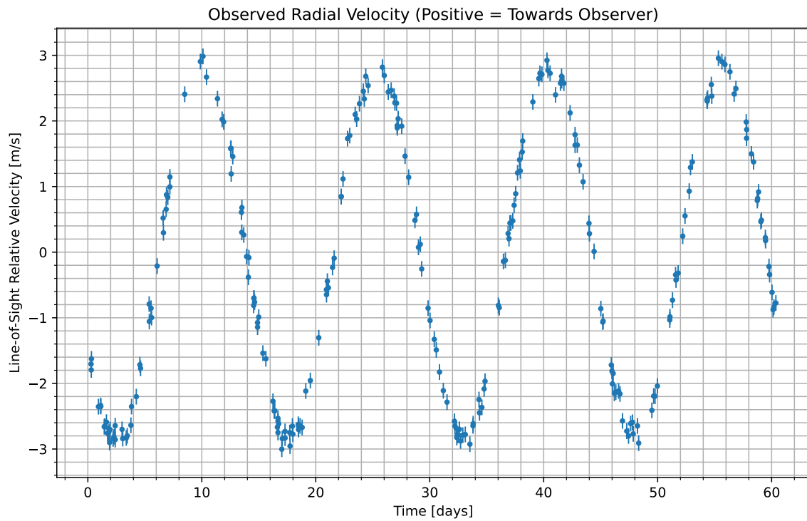
Figure 1: We have isolated the radial velocity of the host star due to the candidate planet. Data begins at UTC 2089-02-19/02:05. Positive values indicate the velocity at which the star is moving towards us; negative indicate the velocity at which it is moving away.
