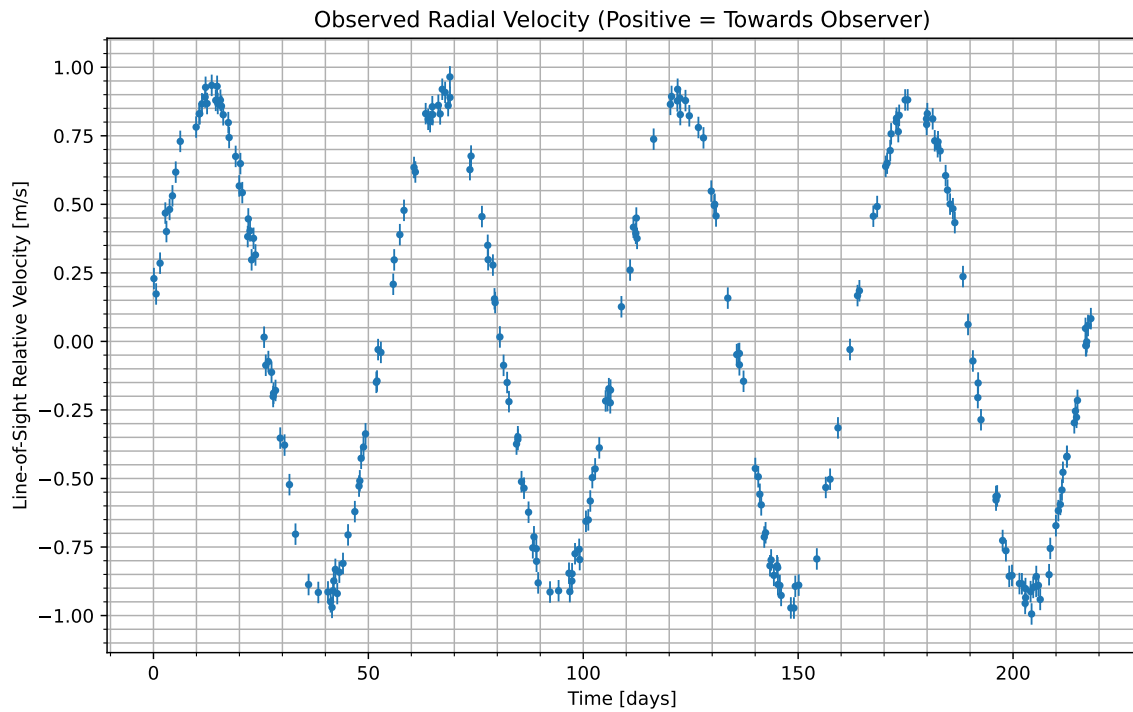
Figure 1: We have isolated the radial velocity of the host star due to the candidate planet. Data begins at UTC 2076-07-25/06:34. Positive values indicate the velocity at which the star is moving towards us; negative indicate the velocity at which it is moving away.
