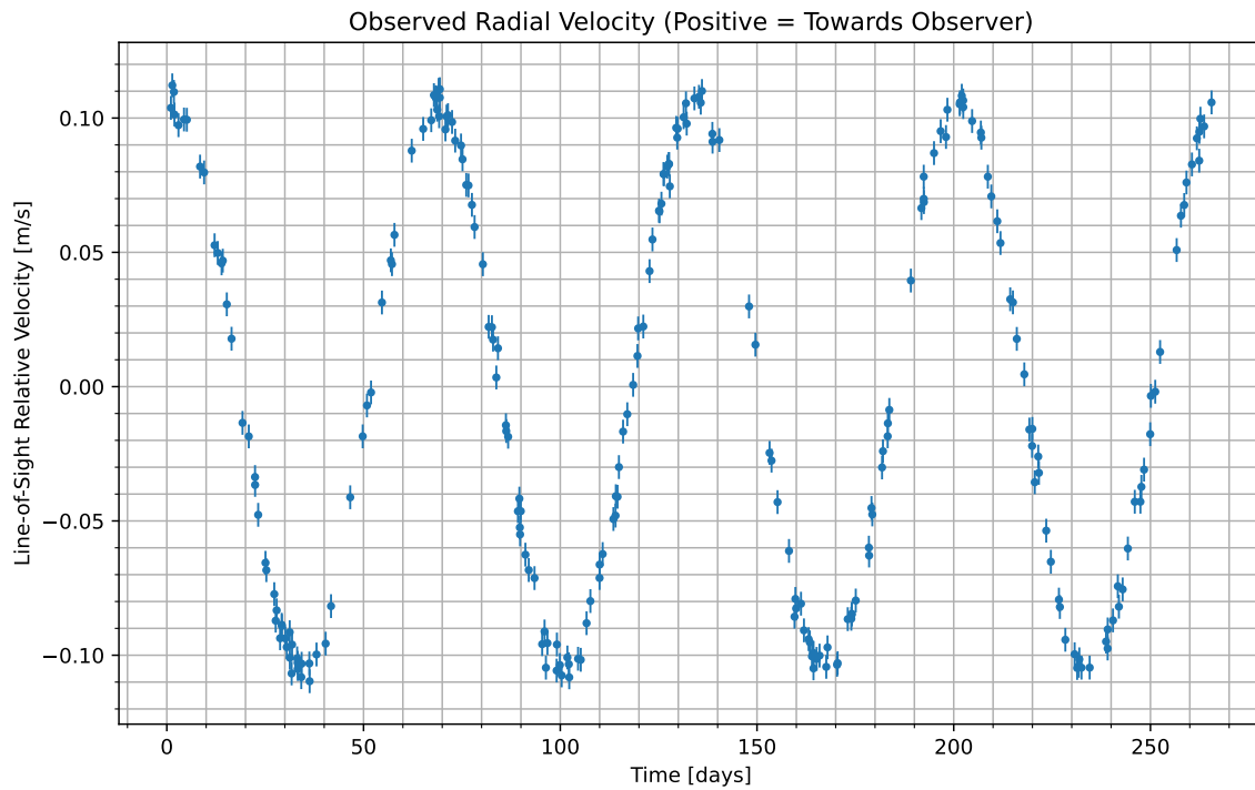
Figure 1: We have isolated the radial velocity of the host star due to the candidate planet. Data begins at UTC 2070-08-18/06:19. Positive values indicate the velocity at which the star is moving towards us; negative indicate the velocity at which it is moving away.
