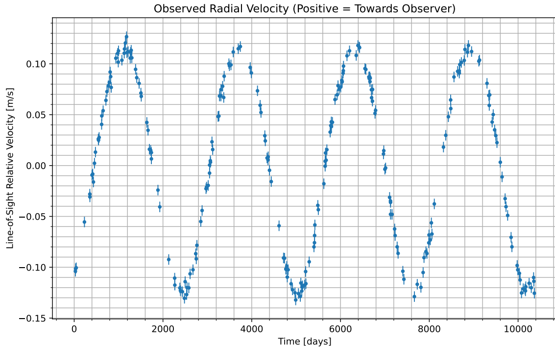
Figure 1: We have isolated the radial velocity of the host star due to the candidate planet. Data begins at UTC 2059-03-15/08:40. Positive values indicate the velocity at which the star is moving towards us; negative indicate the velocity at which it is moving away.
