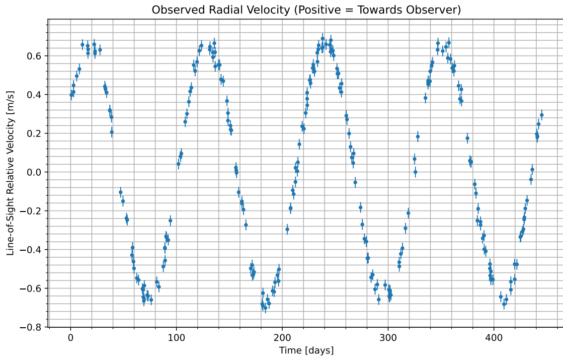
Figure 1: We have isolated the radial velocity of the host star due to the candidate planet. Data begins at UTC 2076-01-28/13:11. Positive values indicate the velocity at which the star is moving towards us; negative indicate the velocity at which it is moving away.
