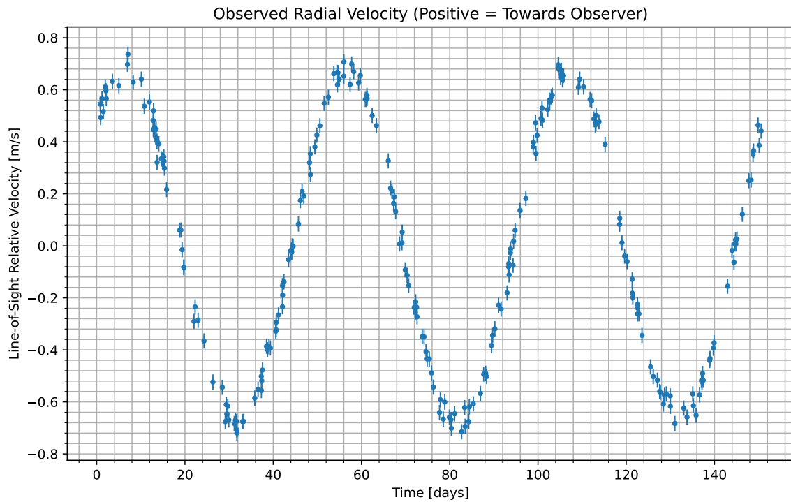
Figure 1: We have isolated the radial velocity of the host star due to the candidate planet. Data begins at UTC 2089-04-19/15:15. Positive values indicate the velocity at which the star is moving towards us; negative indicate the velocity at which it is moving away.
