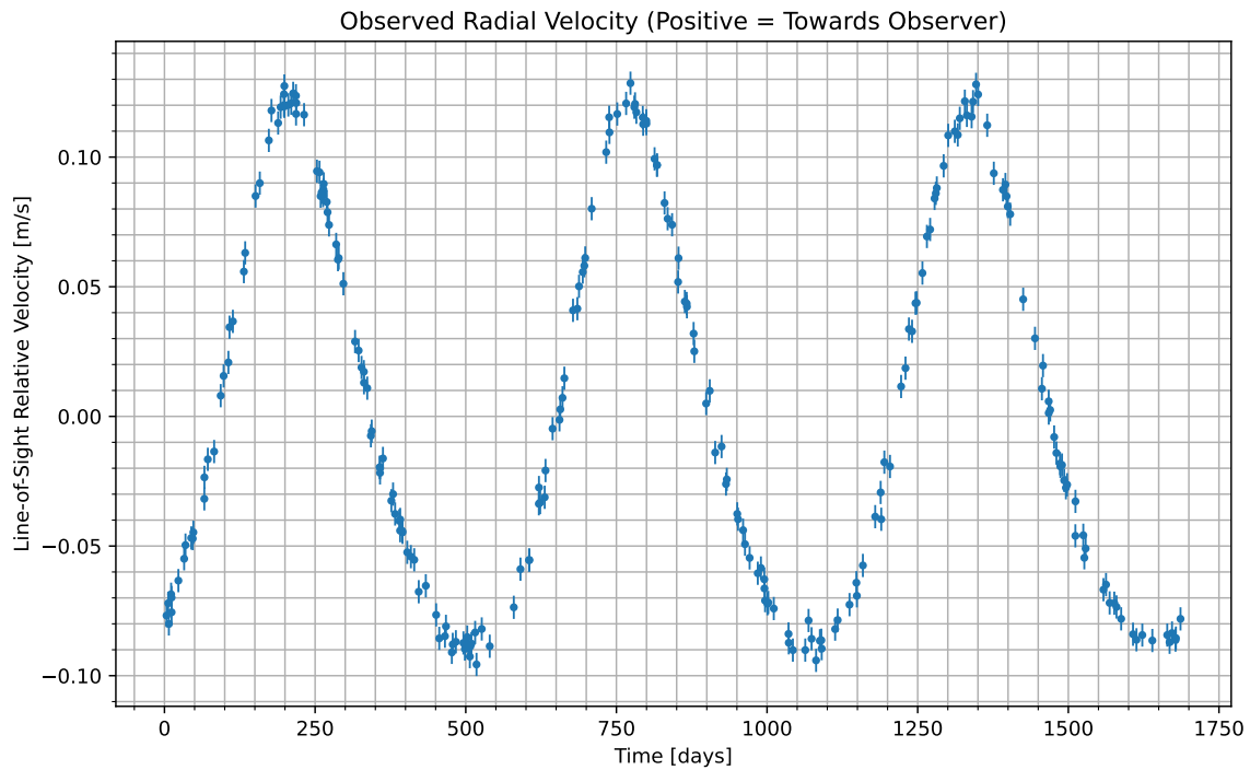
Figure 1: We have isolated the radial velocity of the host star due to the candidate planet. Data begins at UTC 2081-03-15/05:03. Positive values indicate the velocity at which the star is moving towards us; negative indicate the velocity at which it is moving away.
