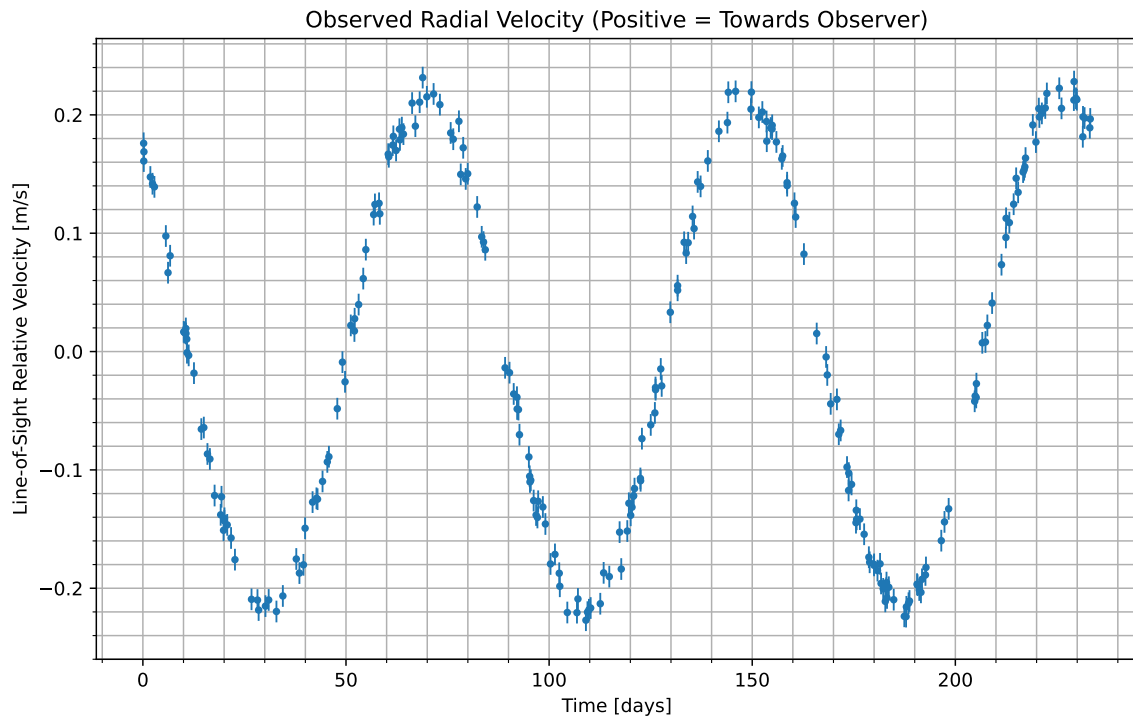
Figure 1: We have isolated the radial velocity of the host star due to the candidate planet. Data begins at UTC 2098-05-08/01:21. Positive values indicate the velocity at which the star is moving towards us; negative indicate the velocity at which it is moving away.
