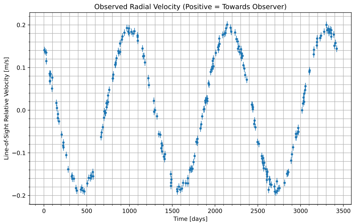
Figure 1: We have isolated the radial velocity of the host star due to the candidate planet. Data begins at UTC 2062-07-23/19:31. Positive values indicate the velocity at which the star is moving towards us; negative indicate the velocity at which it is moving away.
