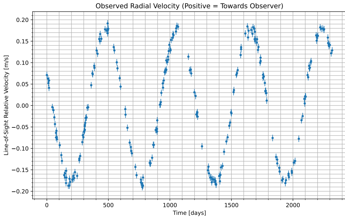
Figure 1: We have isolated the radial velocity of the host star due to the candidate planet. Data begins at UTC 2074-11-15/15:03. Positive values indicate the velocity at which the star is moving towards us; negative indicate the velocity at which it is moving away.
