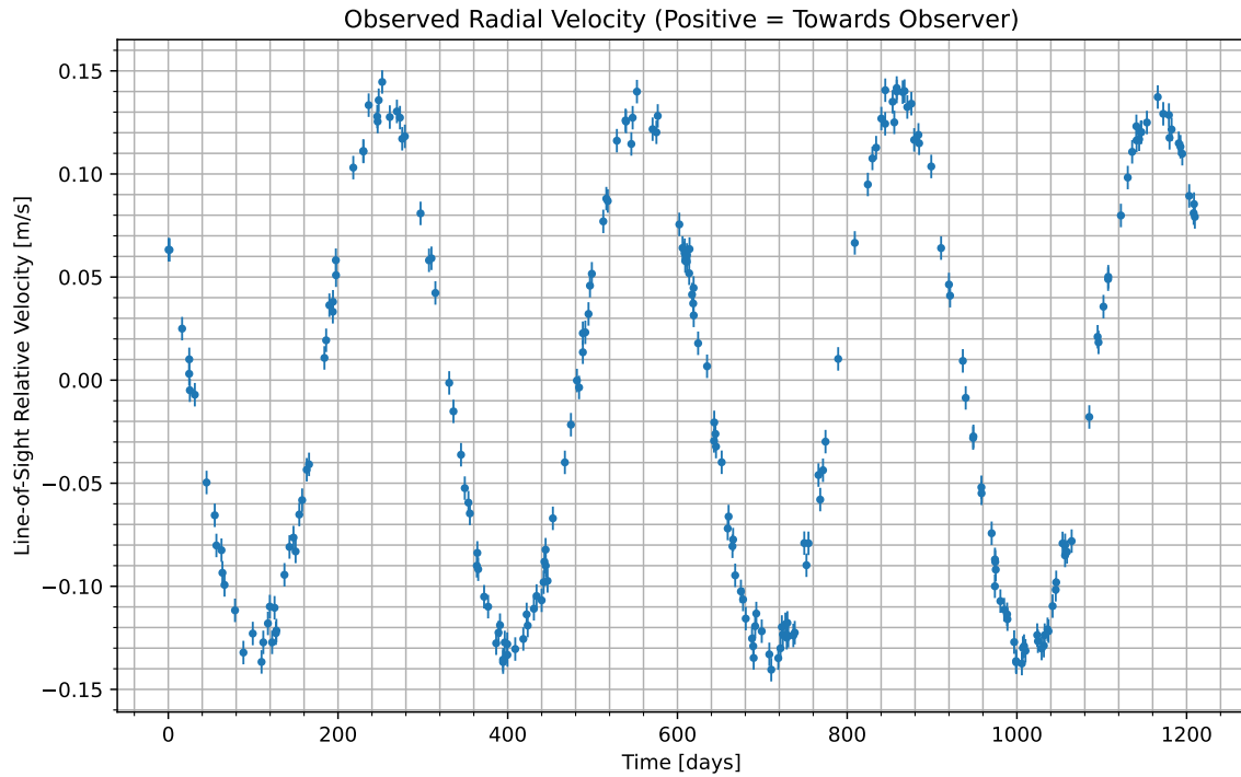
Figure 1: We have isolated the radial velocity of the host star due to the candidate planet. Data begins at UTC 2073-12-30/22:18. Positive values indicate the velocity at which the star is moving towards us; negative indicate the velocity at which it is moving away.
