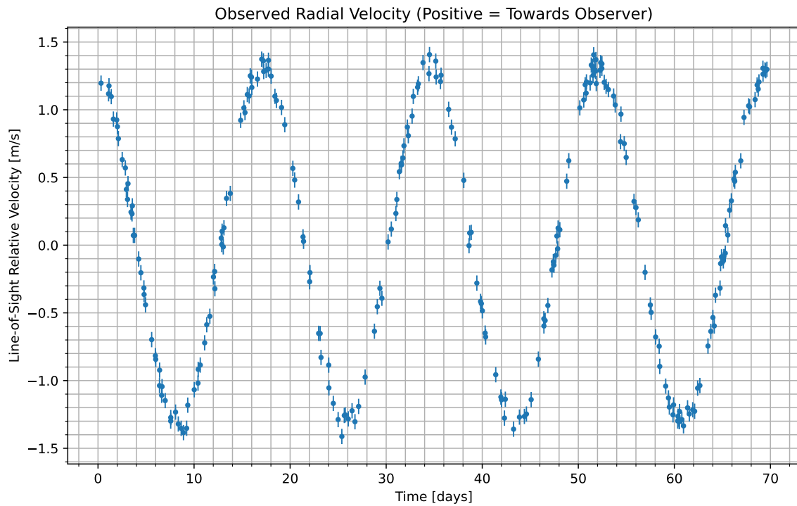
Figure 1: We have isolated the radial velocity of the host star due to the candidate planet. Data begins at UTC 2081-04-10/16:49. Positive values indicate the velocity at which the star is moving towards us; negative indicate the velocity at which it is moving away.
