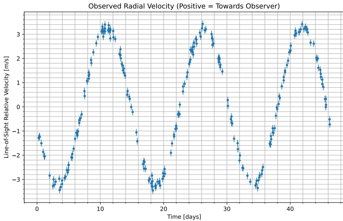
Figure 1: We have isolated the radial velocity of the host star due to the candidate planet. Data begins at UTC 2095-06-23/09:05. Positive values indicate the velocity at which the star is moving towards us; negative indicate the velocity at which it is moving away.
