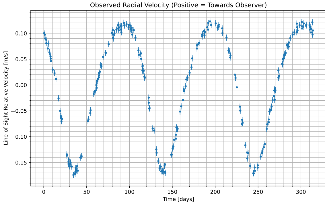
Figure 1: We have isolated the radial velocity of the host star due to the candidate planet. Data begins at UTC 2070-10-22/18:11. Positive values indicate the velocity at which the star is moving towards us; negative indicate the velocity at which it is moving away.
