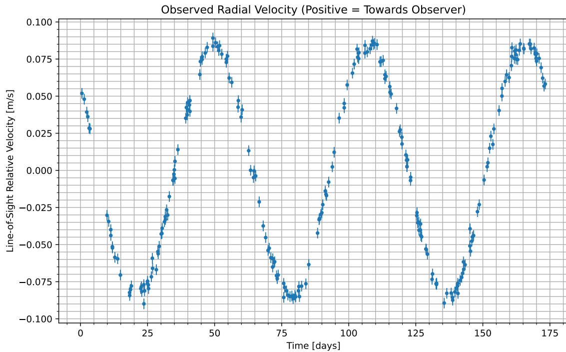
Figure 1: We have isolated the radial velocity of the host star due to the candidate planet. Data begins at UTC 2090-10-31/00:49. Positive values indicate the velocity at which the star is moving towards us; negative indicate the velocity at which it is moving away.
