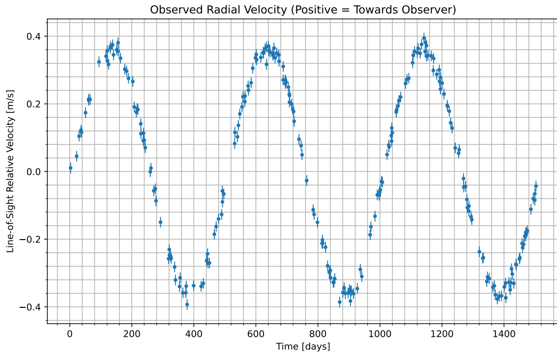
Figure 1: We have isolated the radial velocity of the host star due to the candidate planet. Data begins at UTC 2089-11-20/00:56. Positive values indicate the velocity at which the star is moving towards us; negative indicate the velocity at which it is moving away.
