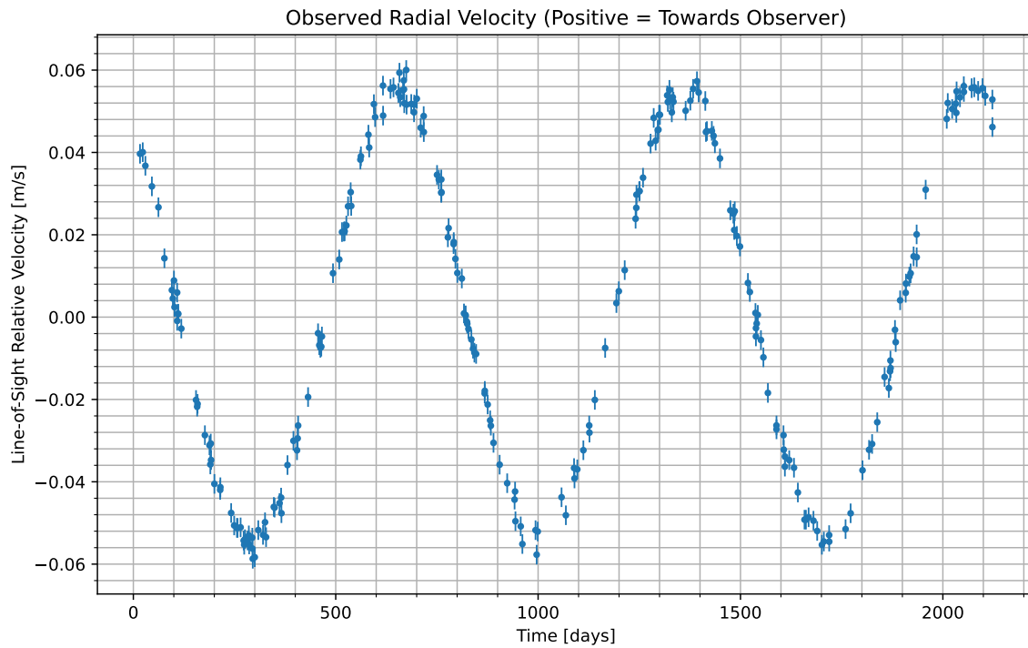
Figure 1: We have isolated the radial velocity of the host star due to the candidate planet. Data begins at UTC 2071-10-09/21:42. Positive values indicate the velocity at which the star is moving towards us; negative indicate the velocity at which it is moving away.
