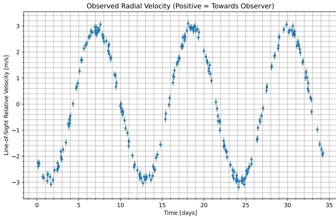
Figure 1: We have isolated the radial velocity of the host star due to the candidate planet. Data begins at UTC 2088-08-27/19:28. Positive values indicate the velocity at which the star is moving towards us; negative indicate the velocity at which it is moving away.
