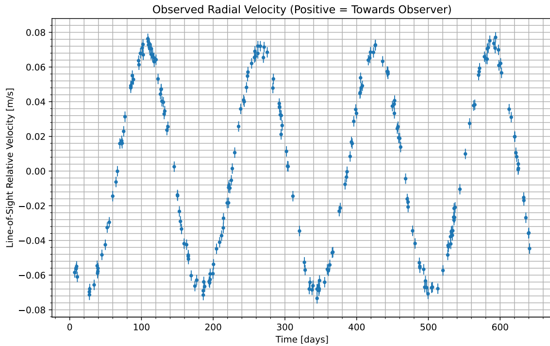
Figure 1: We have isolated the radial velocity of the host star due to the candidate planet. Data begins at UTC 2080-08-05/09:38. Positive values indicate the velocity at which the star is moving towards us; negative indicate the velocity at which it is moving away.
