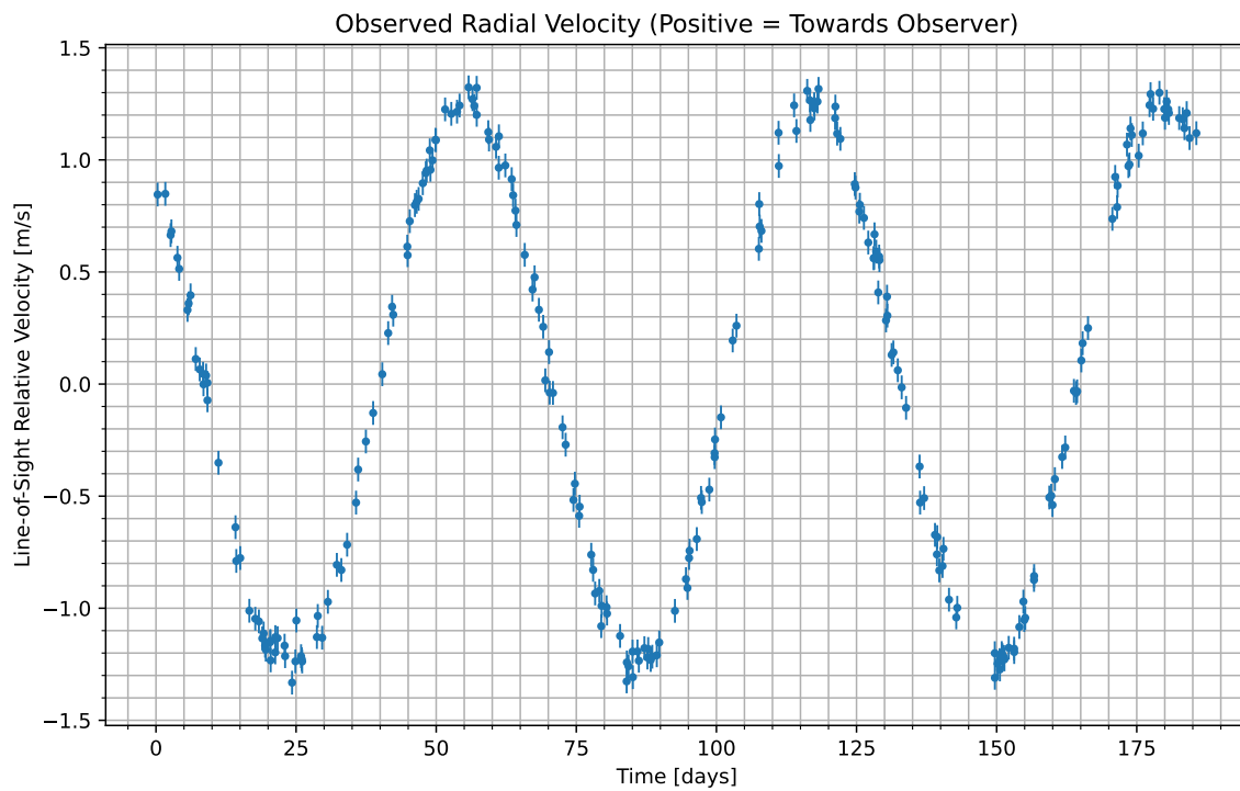
Figure 1: We have isolated the radial velocity of the host star due to the candidate planet. Data begins at UTC 2089-01-14/13:25. Positive values indicate the velocity at which the star is moving towards us; negative indicate the velocity at which it is moving away.
