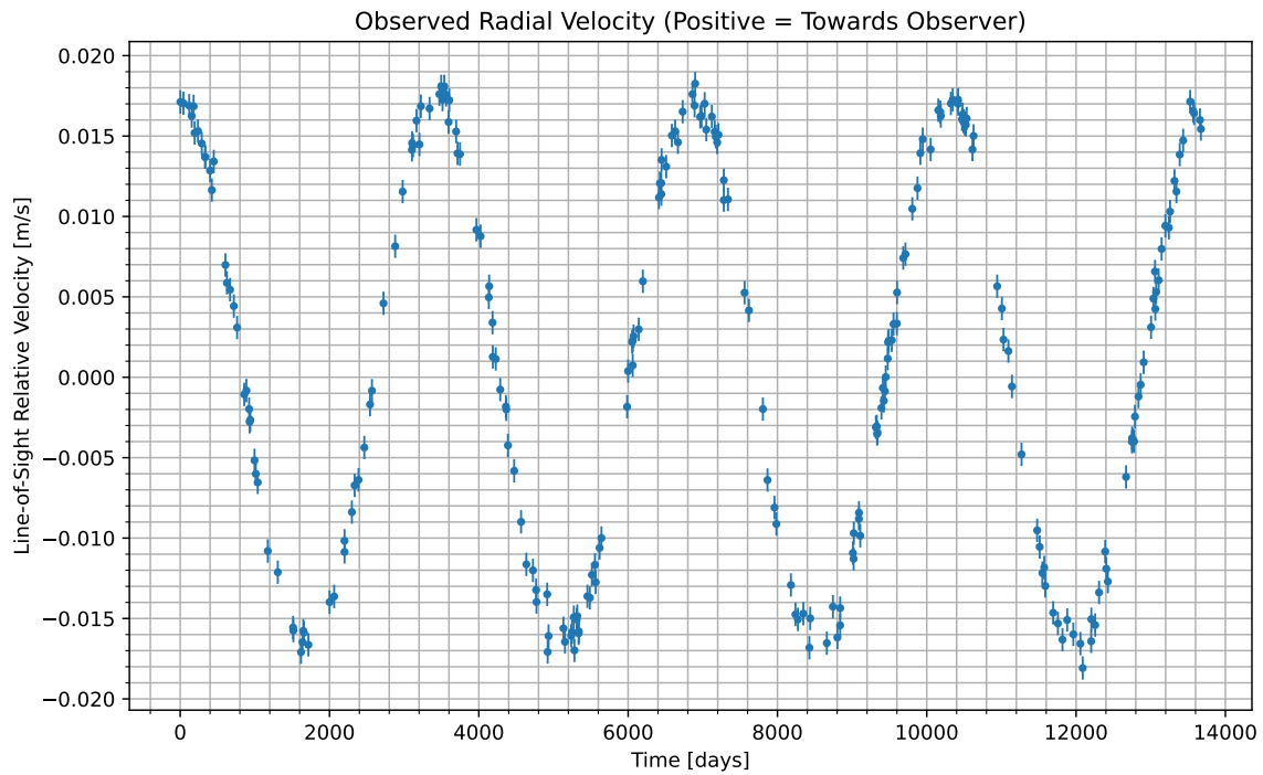
Figure 1: We have isolated the radial velocity of the host star due to the candidate planet. Data begins at UTC 2055-07-11/16:50. Positive values indicate the velocity at which the star is moving towards us; negative indicate the velocity at which it is moving away.
