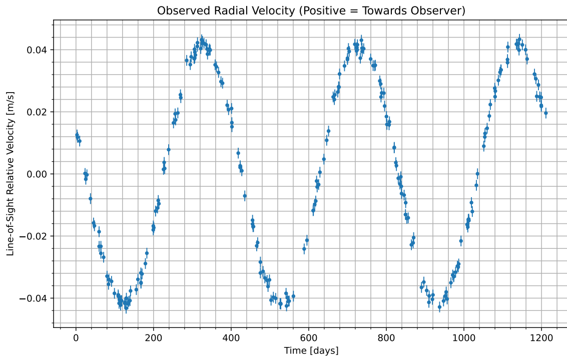
Figure 1: We have isolated the radial velocity of the host star due to the candidate planet. Data begins at UTC 2078-07-30/18:13. Positive values indicate the velocity at which the star is moving towards us; negative indicate the velocity at which it is moving away.
