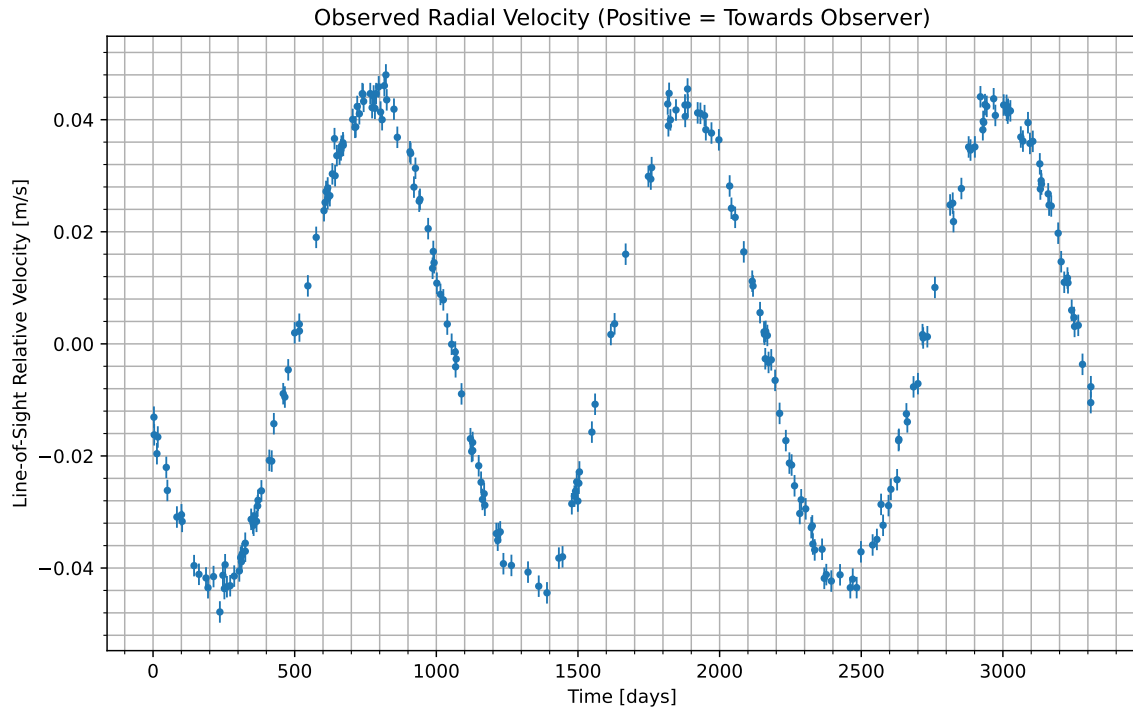
Figure 1: We have isolated the radial velocity of the host star due to the candidate planet. Data begins at UTC 2067-04-22/01:43. Positive values indicate the velocity at which the star is moving towards us; negative indicate the velocity at which it is moving away.
