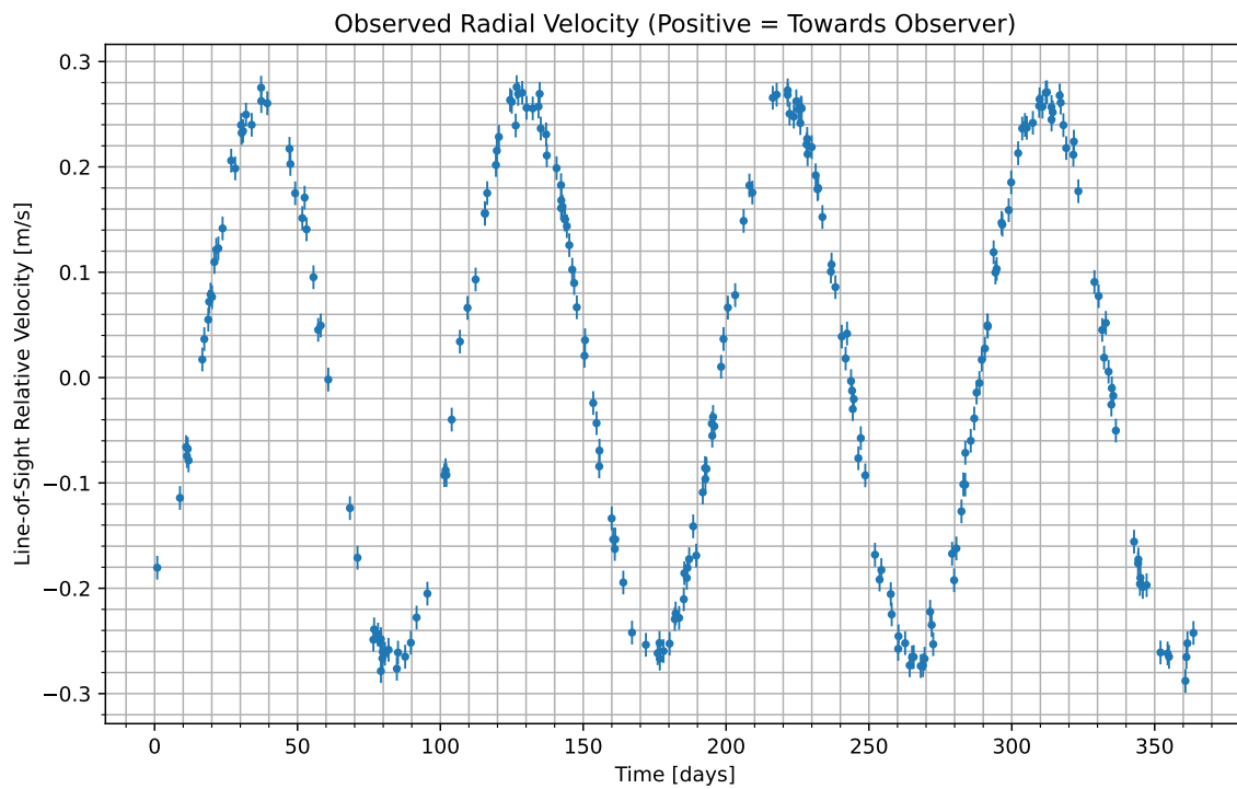
Figure 1: We have isolated the radial velocity of the host star due to the candidate planet. Data begins at UTC 2069-02-24/00:11. Positive values indicate the velocity at which the star is moving towards us; negative indicate the velocity at which it is moving away.
