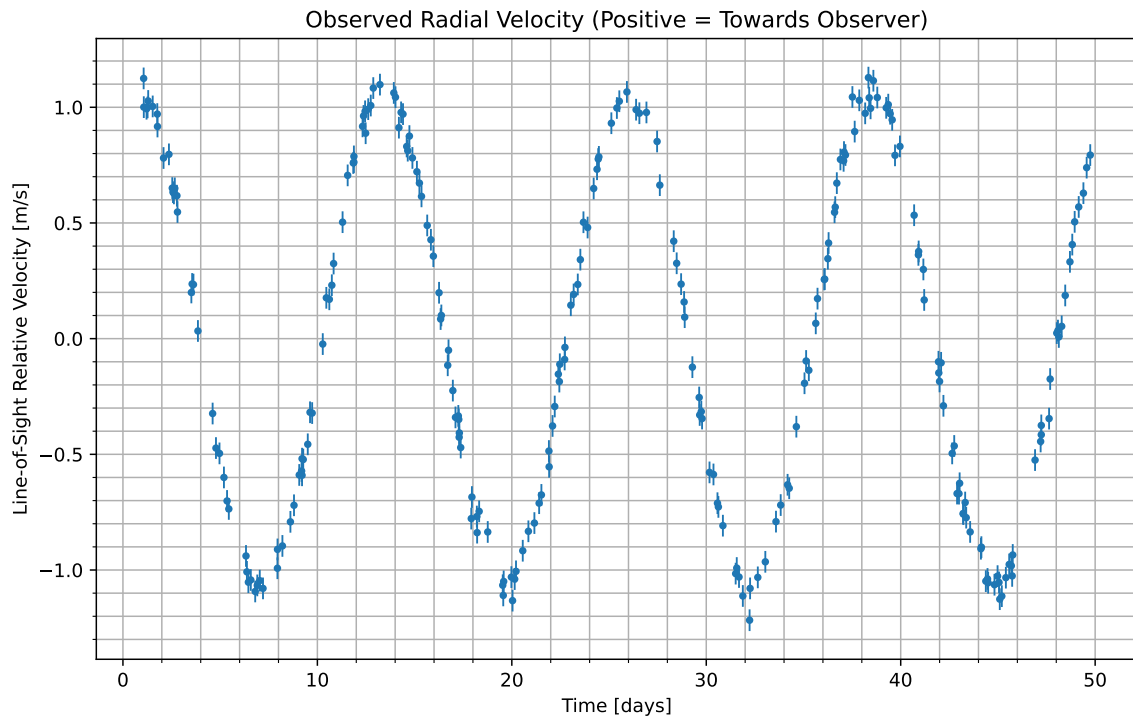
Figure 1: We have isolated the radial velocity of the host star due to the candidate planet. Data begins at UTC 2095-09-15/16:48. Positive values indicate the velocity at which the star is moving towards us; negative indicate the velocity at which it is moving away.
