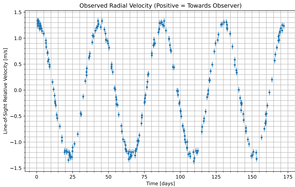
Figure 1: We have isolated the radial velocity of the host star due to the candidate planet. Data begins at UTC 2088-04-23/03:37. Positive values indicate the velocity at which the star is moving towards us; negative indicate the velocity at which it is moving away.
