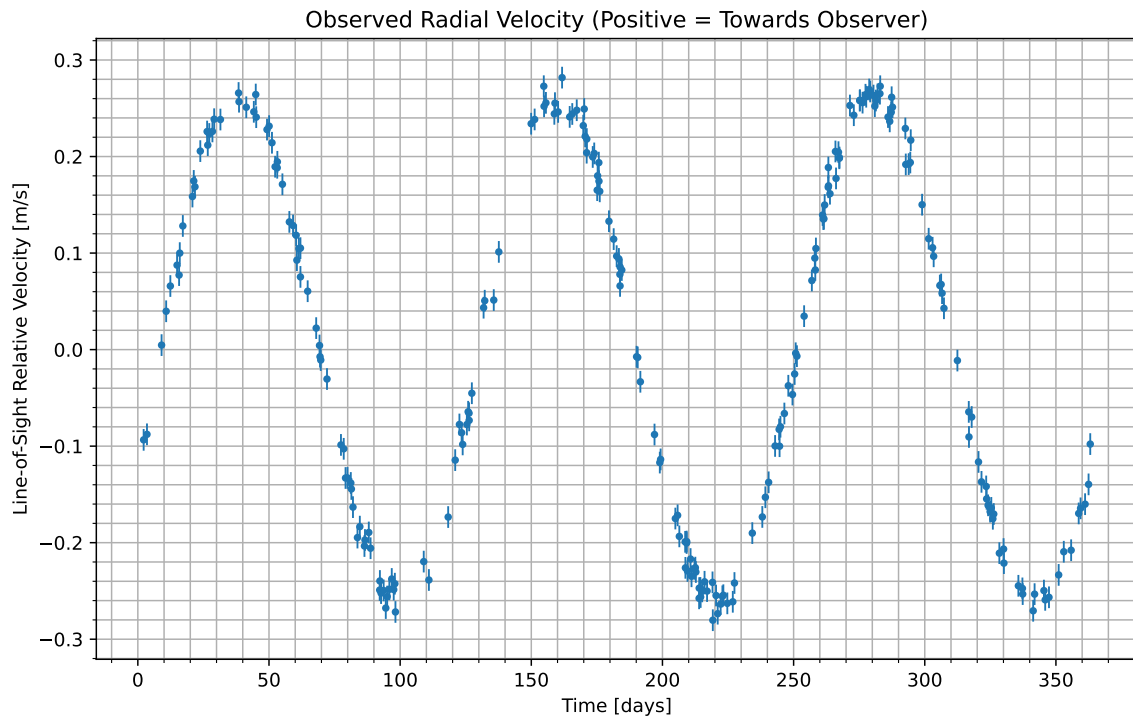
Figure 1: We have isolated the radial velocity of the host star due to the candidate planet. Data begins at UTC 2093-04-14/23:53. Positive values indicate the velocity at which the star is moving towards us; negative indicate the velocity at which it is moving away.
