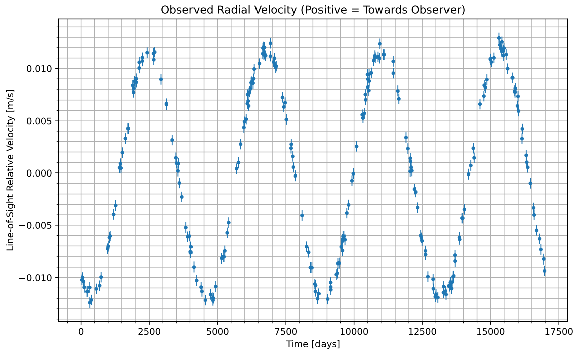
Figure 1: We have isolated the radial velocity of the host star due to the candidate planet. Data begins at UTC 2041-10-21/17:11. Positive values indicate the velocity at which the star is moving towards us; negative indicate the velocity at which it is moving away.
