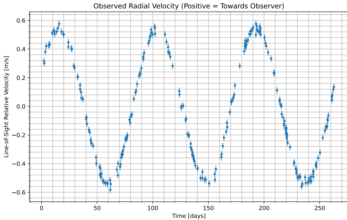
Figure 1: We have isolated the radial velocity of the host star due to the candidate planet. Data begins at UTC 2088-04-02/03:17. Positive values indicate the velocity at which the star is moving towards us; negative indicate the velocity at which it is moving away.
