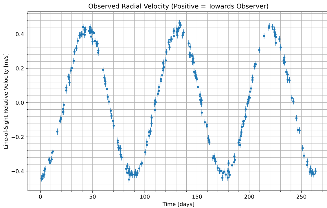
Figure 1: We have isolated the radial velocity of the host star due to the candidate planet. Data begins at UTC 2097-04-30/07:44. Positive values indicate the velocity at which the star is moving towards us; negative indicate the velocity at which it is moving away.
