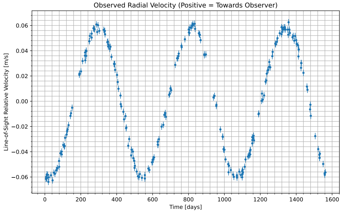
Figure 1: We have isolated the radial velocity of the host star due to the candidate planet. Data begins at UTC 2084-02-07/16:54. Positive values indicate the velocity at which the star is moving towards us; negative indicate the velocity at which it is moving away.
