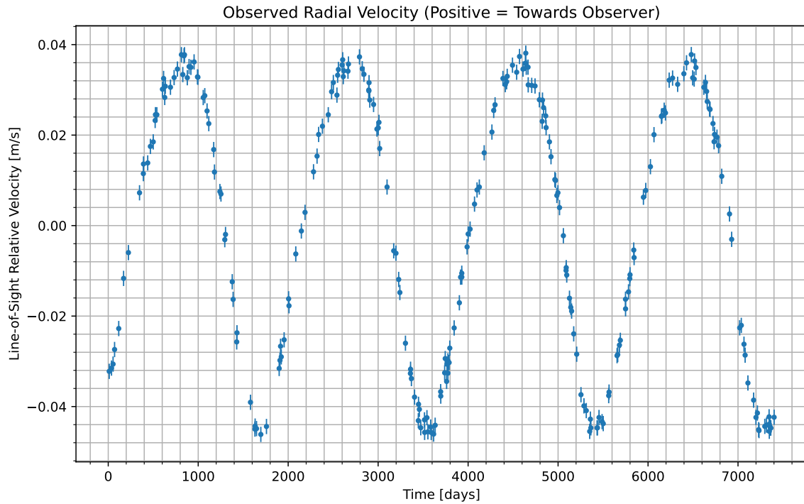
Figure 1: We have isolated the radial velocity of the host star due to the candidate planet. Data begins at UTC 2075-06-10/16:54. Positive values indicate the velocity at which the star is moving towards us; negative indicate the velocity at which it is moving away.
