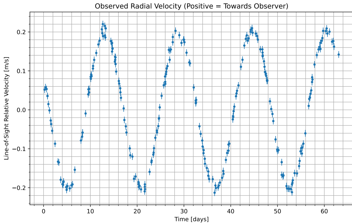
Figure 1: We have isolated the radial velocity of the host star due to the candidate planet. Data begins at UTC 2081-01-13/02:14. Positive values indicate the velocity at which the star is moving towards us; negative indicate the velocity at which it is moving away.
