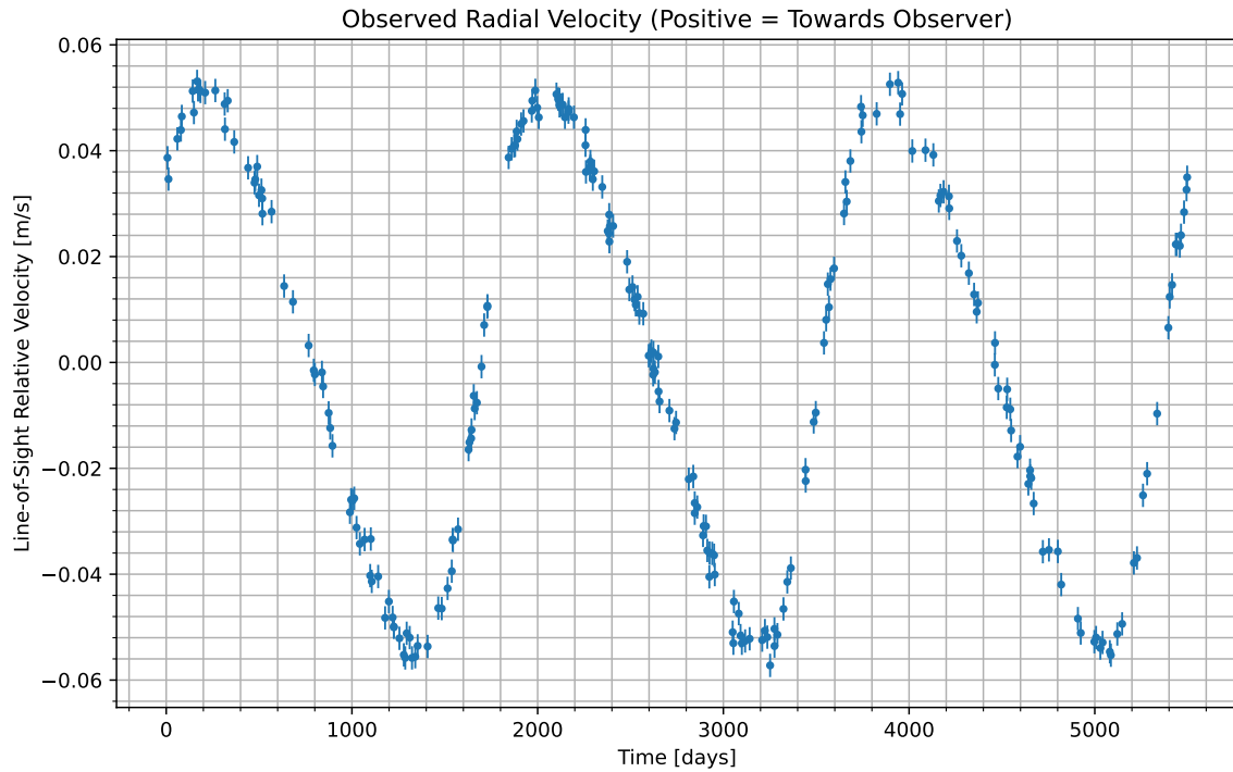
Figure 1: We have isolated the radial velocity of the host star due to the candidate planet. Data begins at UTC 2084-05-11/21:52. Positive values indicate the velocity at which the star is moving towards us; negative indicate the velocity at which it is moving away.
