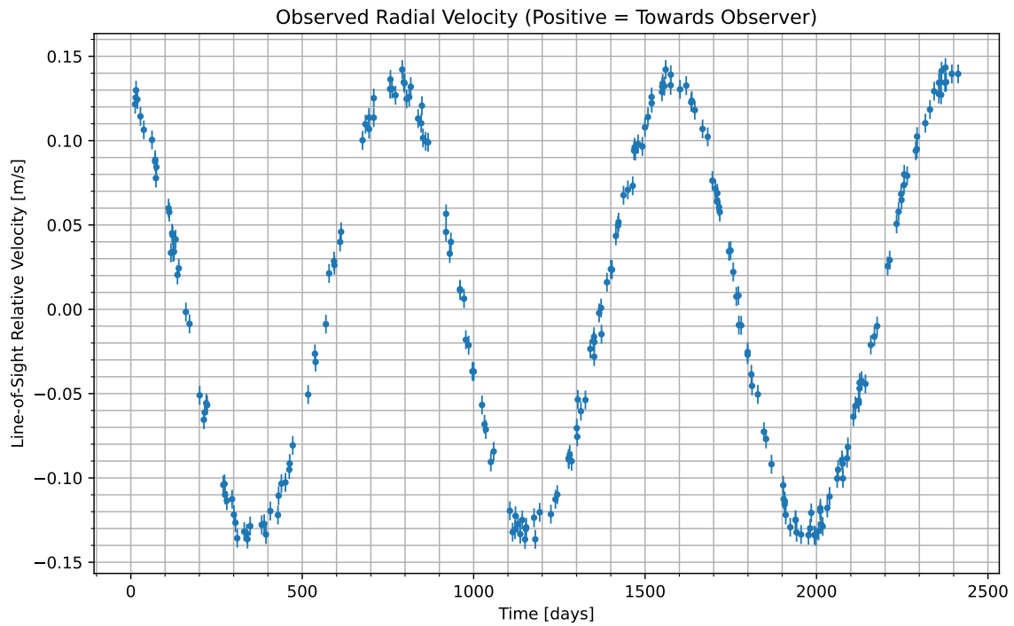
Figure 1: We have isolated the radial velocity of the host star due to the candidate planet. Data begins at UTC 2087-05-24/08:04. Positive values indicate the velocity at which the star is moving towards us; negative indicate the velocity at which it is moving away.
