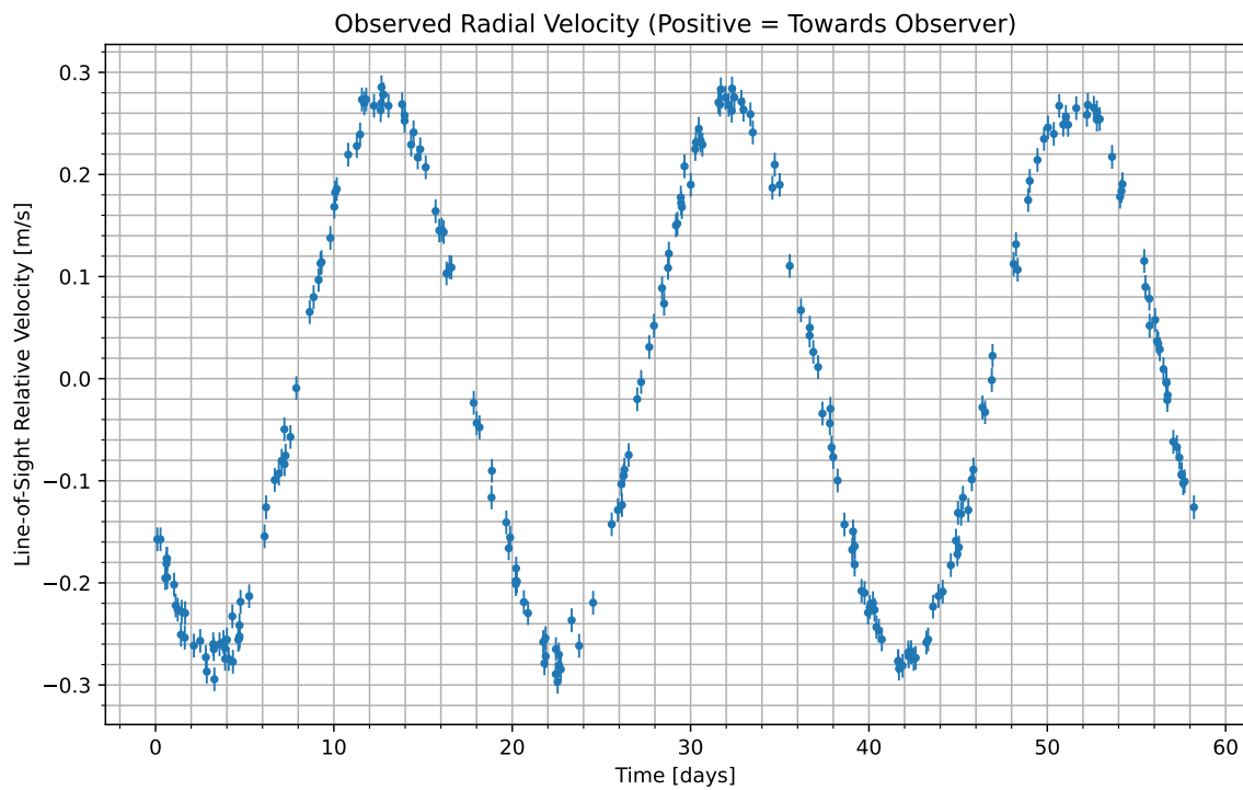
Figure 1: We have isolated the radial velocity of the host star due to the candidate planet. Data begins at UTC 2084-12-11/07:12. Positive values indicate the velocity at which the star is moving towards us; negative indicate the velocity at which it is moving away.
