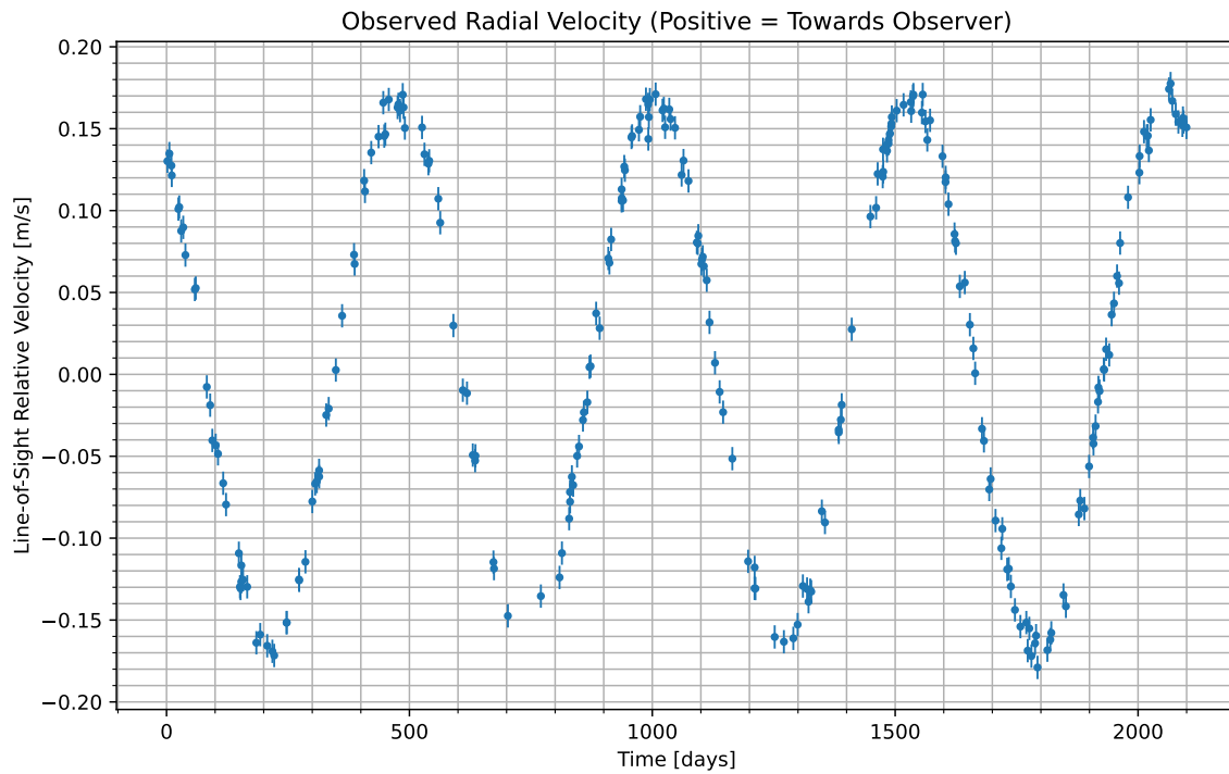
Figure 1: We have isolated the radial velocity of the host star due to the candidate planet. Data begins at UTC 2069-04-21/22:02. Positive values indicate the velocity at which the star is moving towards us; negative indicate the velocity at which it is moving away.
