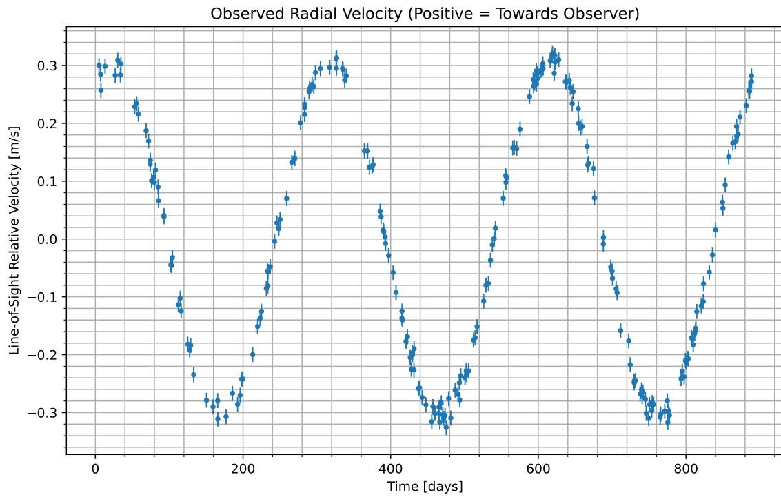
Figure 1: We have isolated the radial velocity of the host star due to the candidate planet. Data begins at UTC 2079-09-16/10:25. Positive values indicate the velocity at which the star is moving towards us; negative indicate the velocity at which it is moving away.
