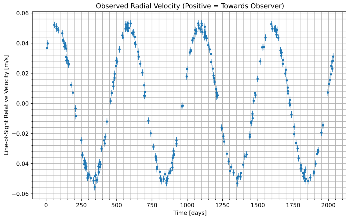
Figure 1: We have isolated the radial velocity of the host star due to the candidate planet. Data begins at UTC 2077-12-10/08:51. Positive values indicate the velocity at which the star is moving towards us; negative indicate the velocity at which it is moving away.
