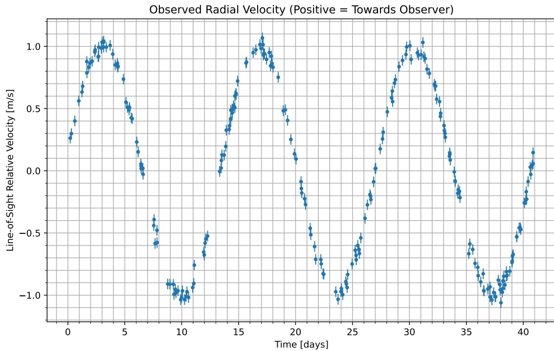
Figure 1: We have isolated the radial velocity of the host star due to the candidate planet. Data begins at UTC 2096-09-22/19:25. Positive values indicate the velocity at which the star is moving towards us; negative indicate the velocity at which it is moving away.
