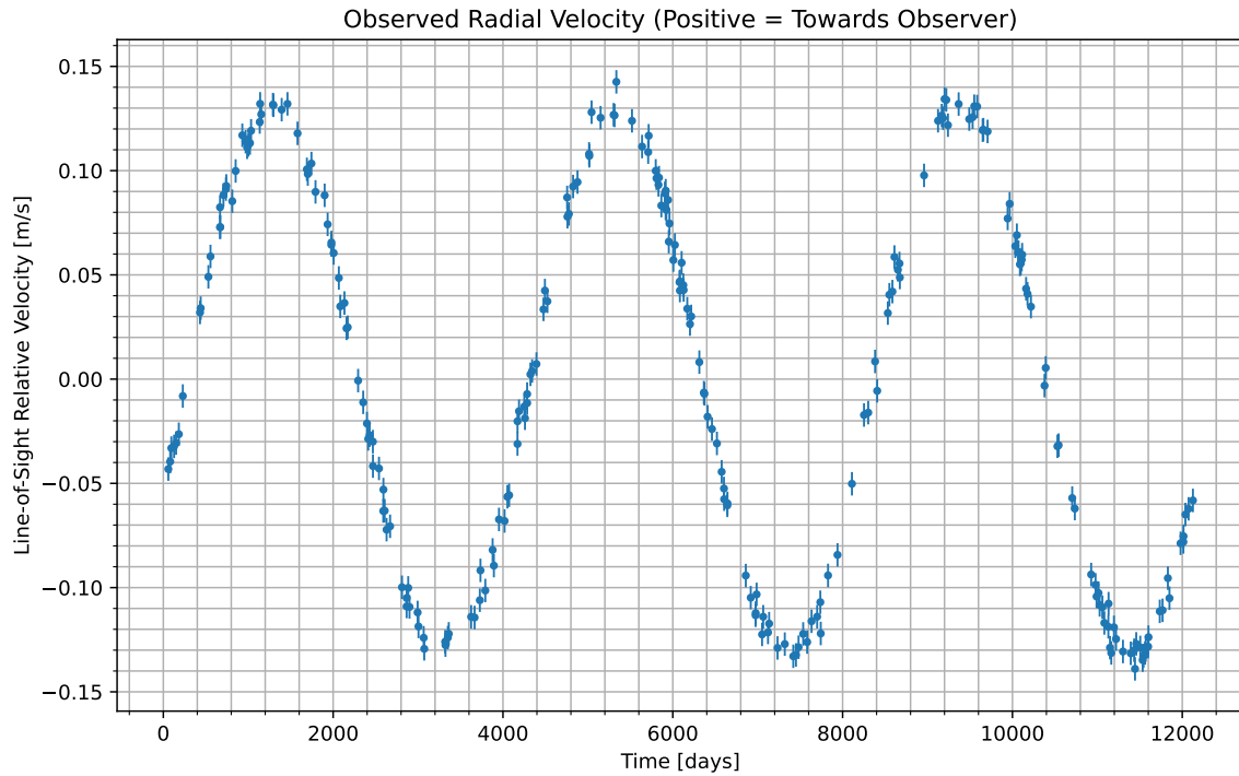
Figure 1: We have isolated the radial velocity of the host star due to the candidate planet. Data begins at UTC 2052-09-19/08:26. Positive values indicate the velocity at which the star is moving towards us; negative indicate the velocity at which it is moving away.
