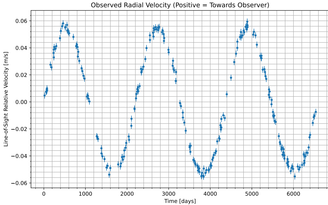
Figure 1: We have isolated the radial velocity of the host star due to the candidate planet. Data begins at UTC 2066-03-21/18:01. Positive values indicate the velocity at which the star is moving towards us; negative indicate the velocity at which it is moving away.
