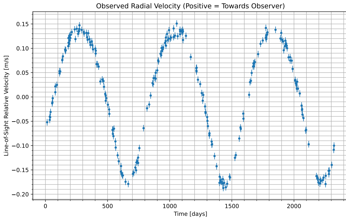
Figure 1: We have isolated the radial velocity of the host star due to the candidate planet. Data begins at UTC 2085-05-28/06:18. Positive values indicate the velocity at which the star is moving towards us; negative indicate the velocity at which it is moving away.
