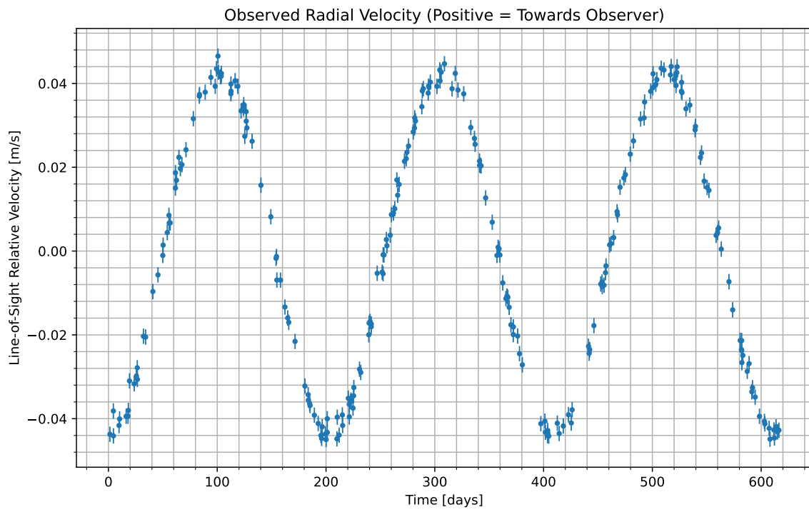
Figure 1: We have isolated the radial velocity of the host star due to the candidate planet. Data begins at UTC 2072-09-09/05:35. Positive values indicate the velocity at which the star is moving towards us; negative indicate the velocity at which it is moving away.
