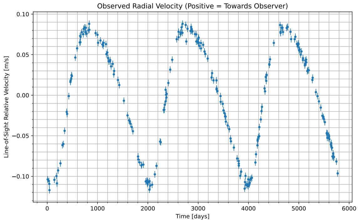
Figure 1: We have isolated the radial velocity of the host star due to the candidate planet. Data begins at UTC 2080-03-21/13:22. Positive values indicate the velocity at which the star is moving towards us; negative indicate the velocity at which it is moving away.
