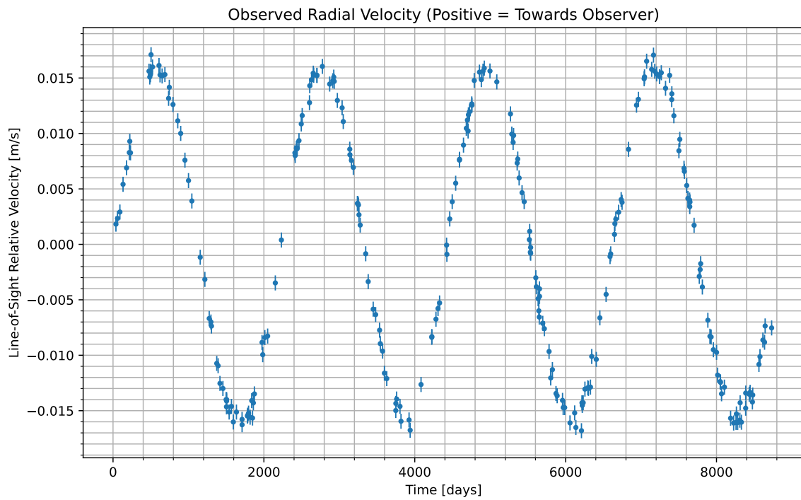
Figure 1: We have isolated the radial velocity of the host star due to the candidate planet. Data begins at UTC 2071-01-14/10:24. Positive values indicate the velocity at which the star is moving towards us; negative indicate the velocity at which it is moving away.
